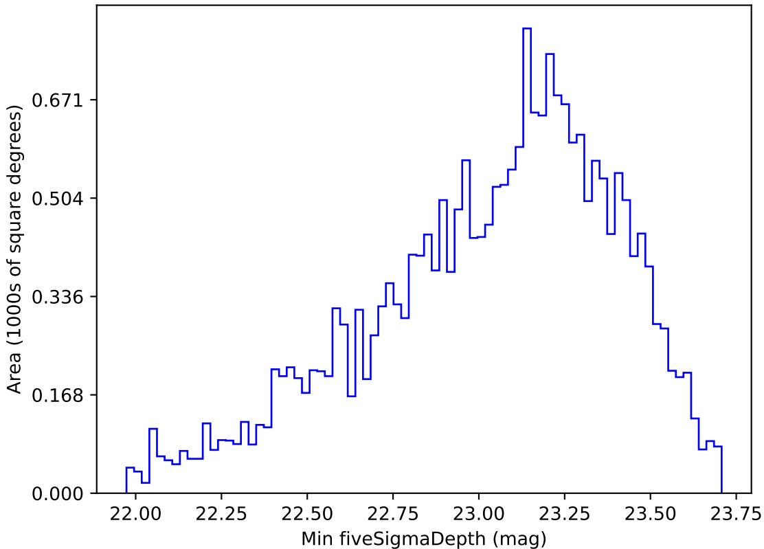
telescope_jerk_v3.5_10yrs Yr 1 u band: Min fiveSigmaDepth
