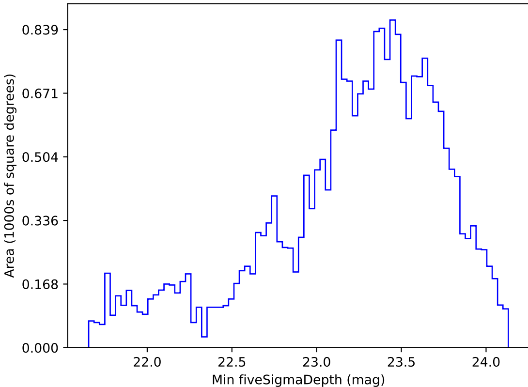
telescope_jerk_v3.5_10yrs Yr 1 r band: Min fiveSigmaDepth
