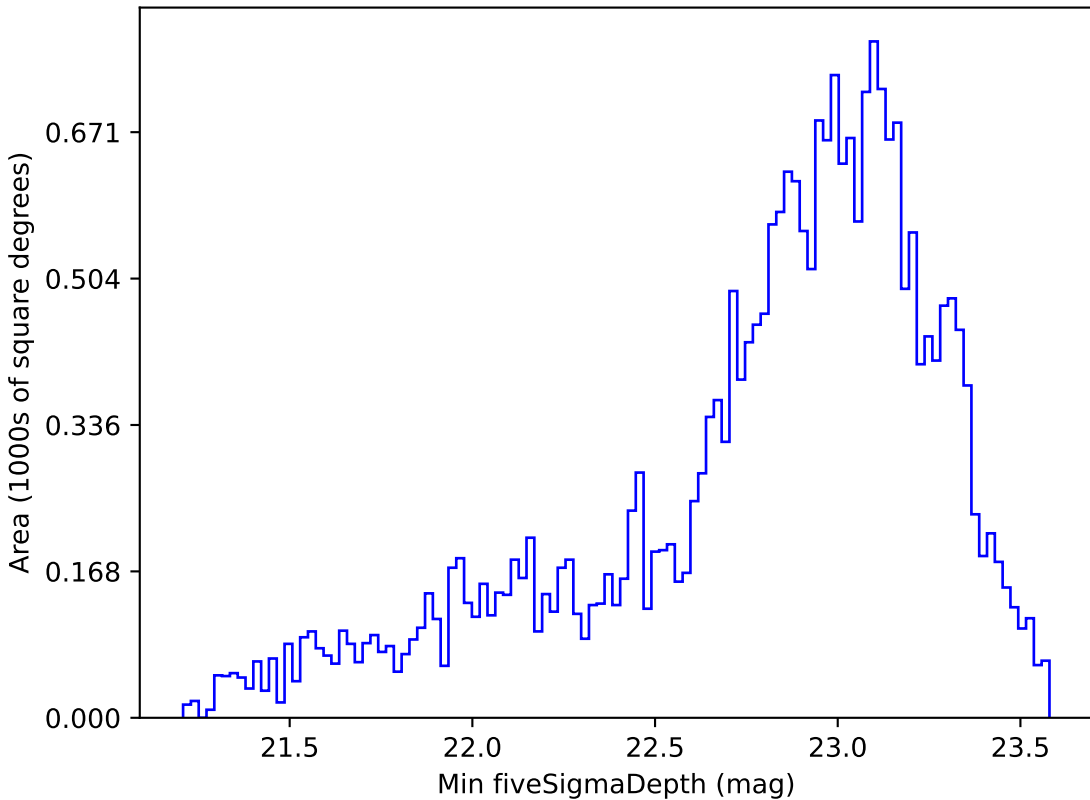
telescope_jerk_v3.5_10yrs Yr 1 i band: Min fiveSigmaDepth
