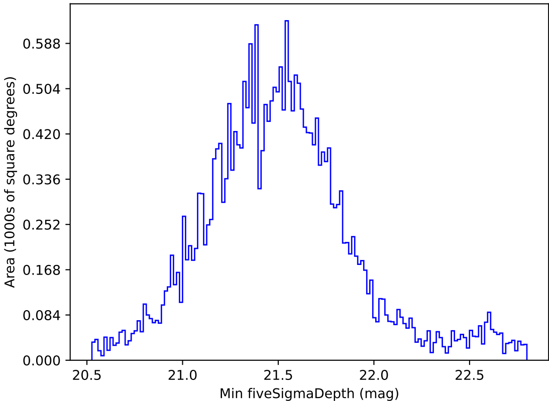
telescope_jerk_v3.5_10yrs Yr 1 all bands: Min fiveSigmaDepth
