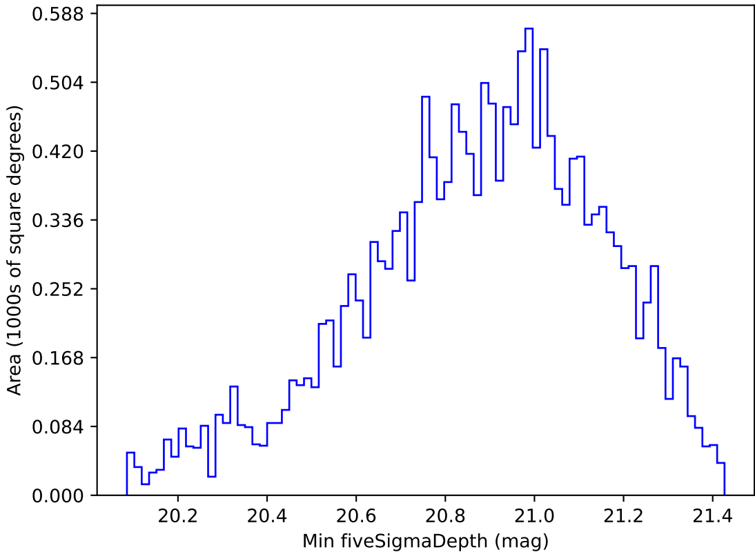
telescope_jerk_v3.5_10yrs WFD y band: Min fiveSigmaDepth
