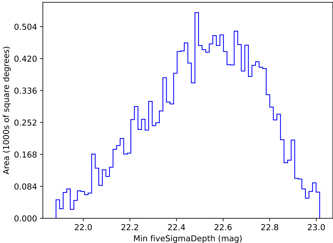
telescope_jerk_v3.5_10yrs WFD u band: Min fiveSigmaDepth
