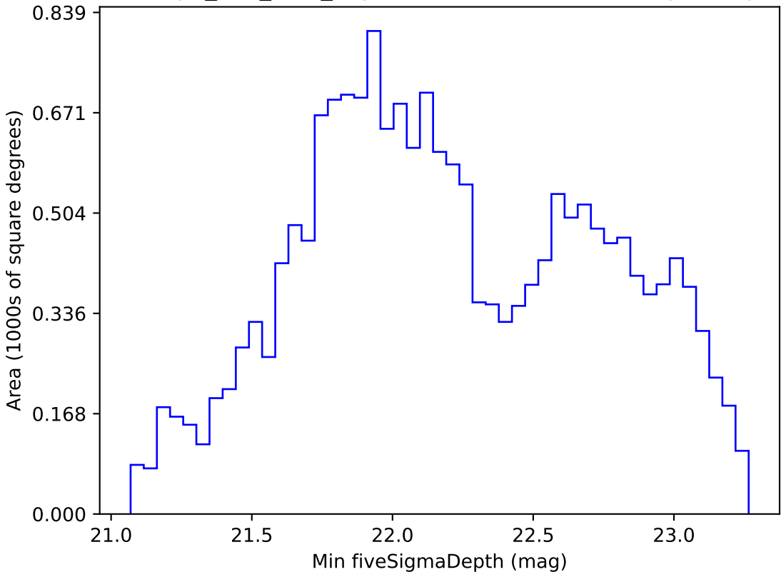
telescope_jerk_v3.5_10yrs WFD r band: Min fiveSigmaDepth
