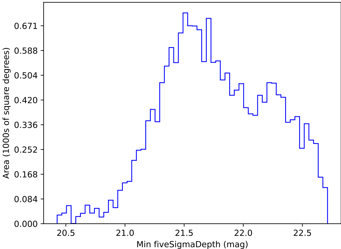
telescope_jerk_v3.5_10yrs WFD i band: Min fiveSigmaDepth
