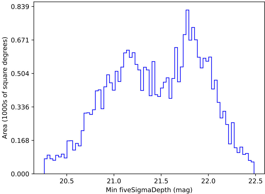
telescope_jerk_v3.5_10yrs All sky z band: Min fiveSigmaDepth
