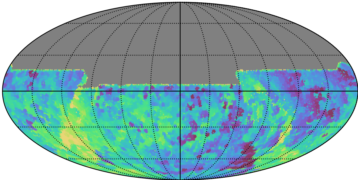
telescope_jerk_v3.5_10yrs All sky y band: Min fiveSigmaDepth
