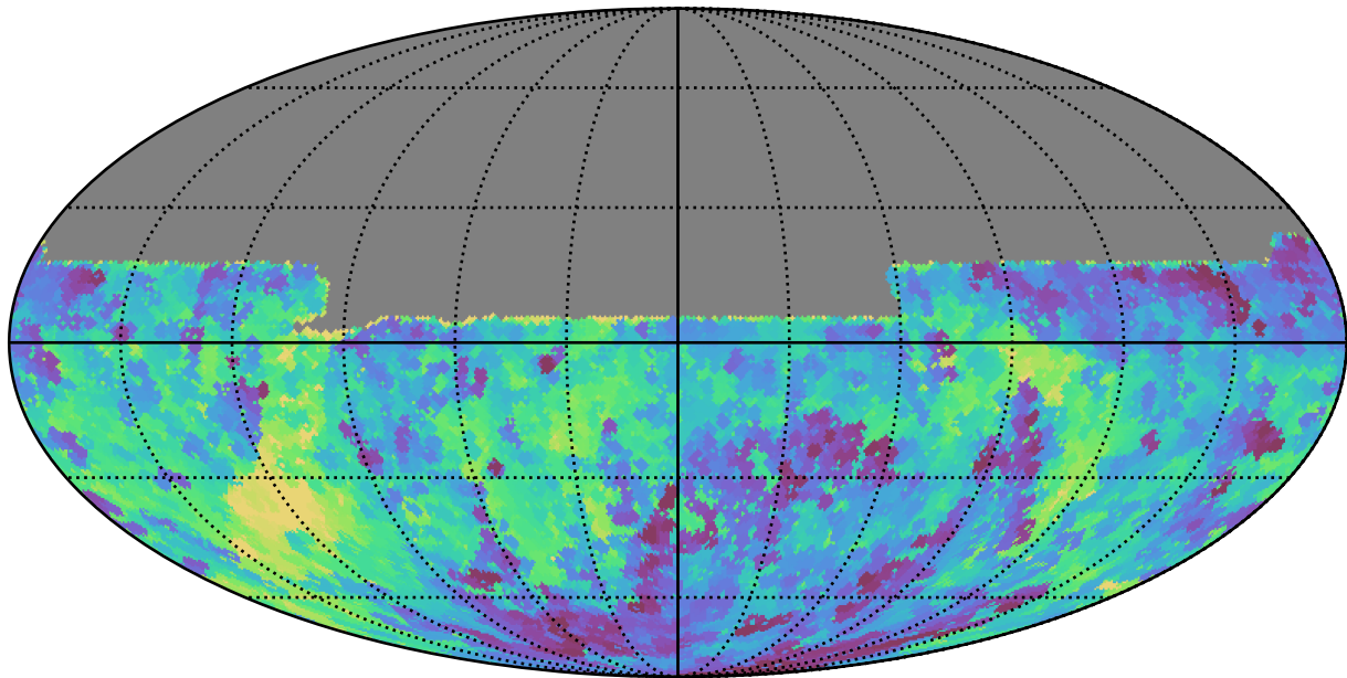
telescope_jerk_v3.5_10yrs All sky u band: Min fiveSigmaDepth
