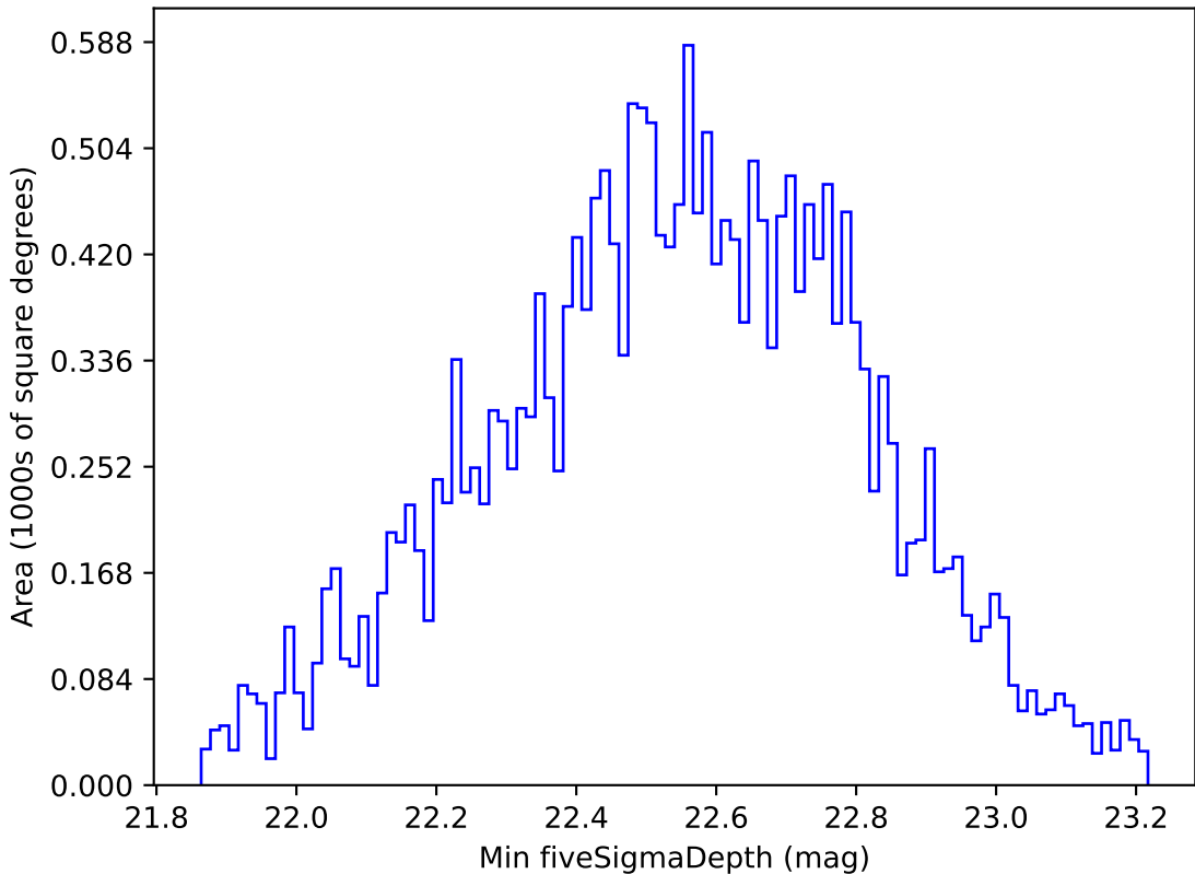
telescope_jerk_v3.5_10yrs All sky u band: Min fiveSigmaDepth
