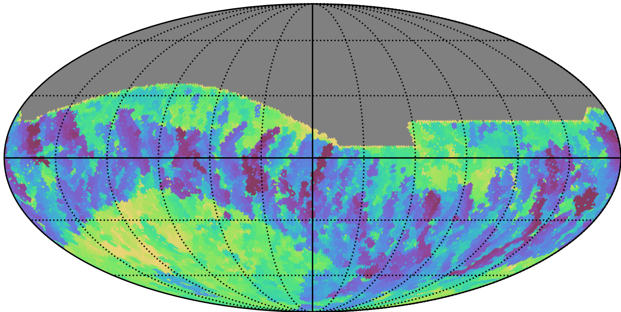
telescope_jerk_v3.5_10yrs All sky r band: Min fiveSigmaDepth
