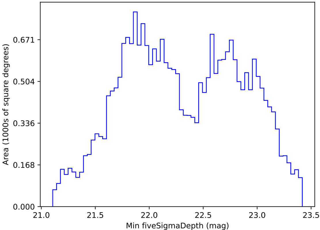
telescope_jerk_v3.5_10yrs All sky r band: Min fiveSigmaDepth
