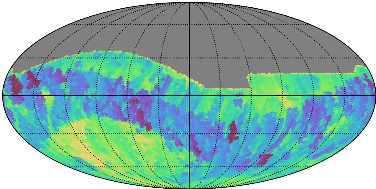
telescope_jerk_v3.5_10yrs All sky i band: Min fiveSigmaDepth
