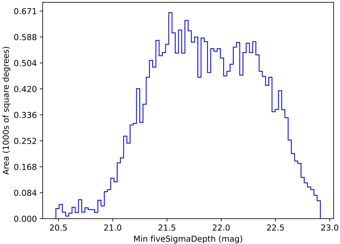
telescope_jerk_v3.5_10yrs All sky i band: Min fiveSigmaDepth
