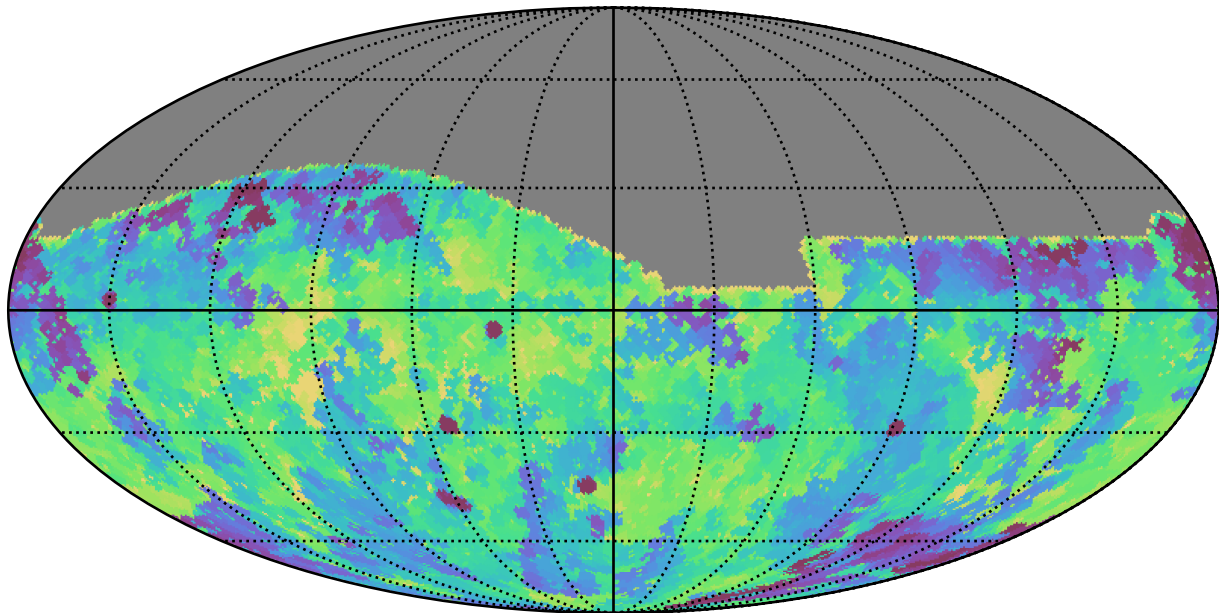
telescope_jerk_v3.5_10yrs All sky g band: Min fiveSigmaDepth
