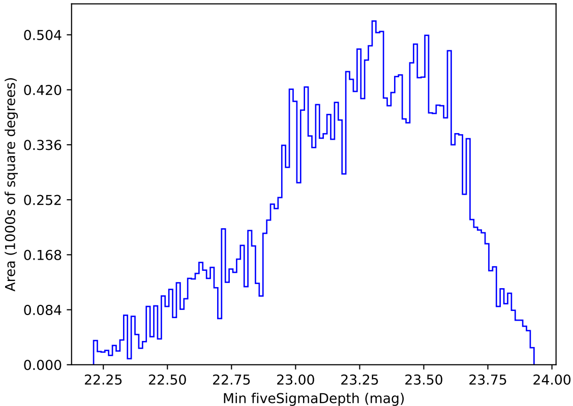
telescope_jerk_v3.5_10yrs All sky g band: Min fiveSigmaDepth
