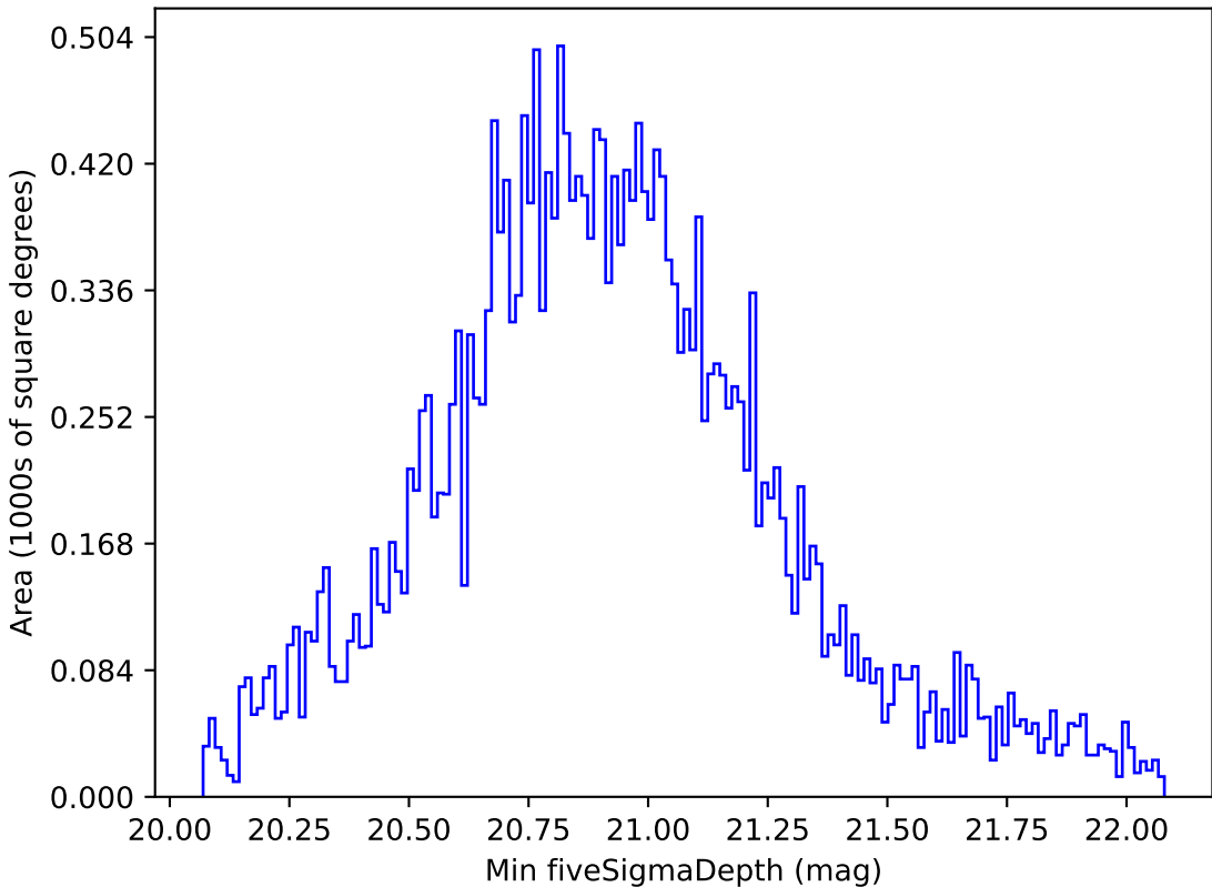
telescope_jerk_v3.5_10yrs All sky all bands: Min fiveSigmaDepth
