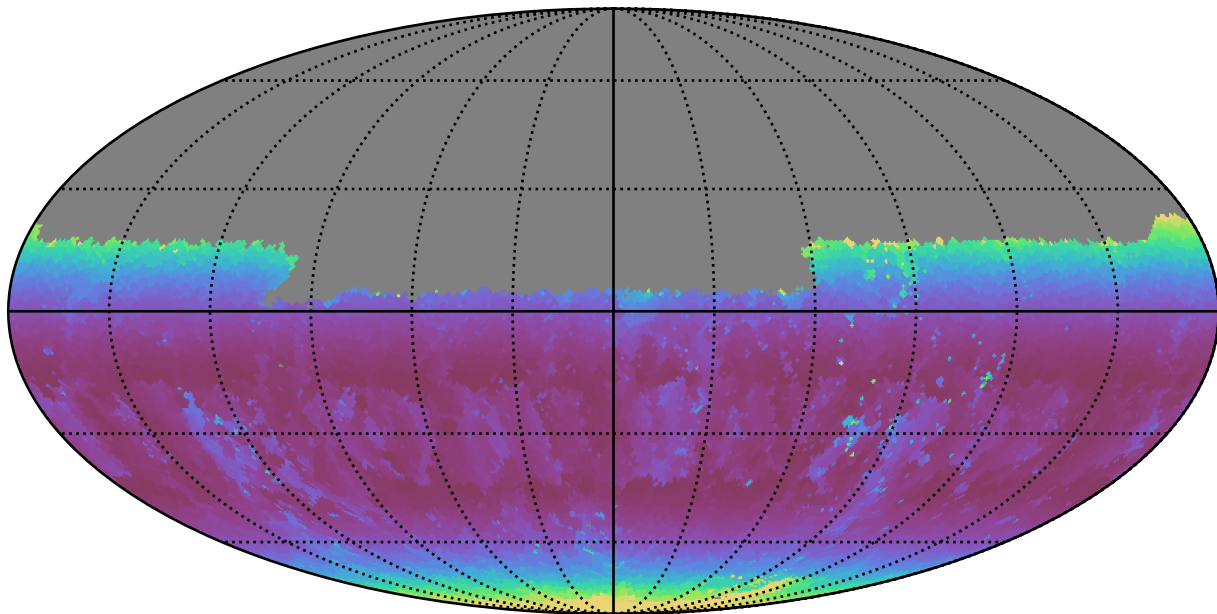
telescope_jerk_v3.5_10yrs Yr 1 u band: Min airmass
