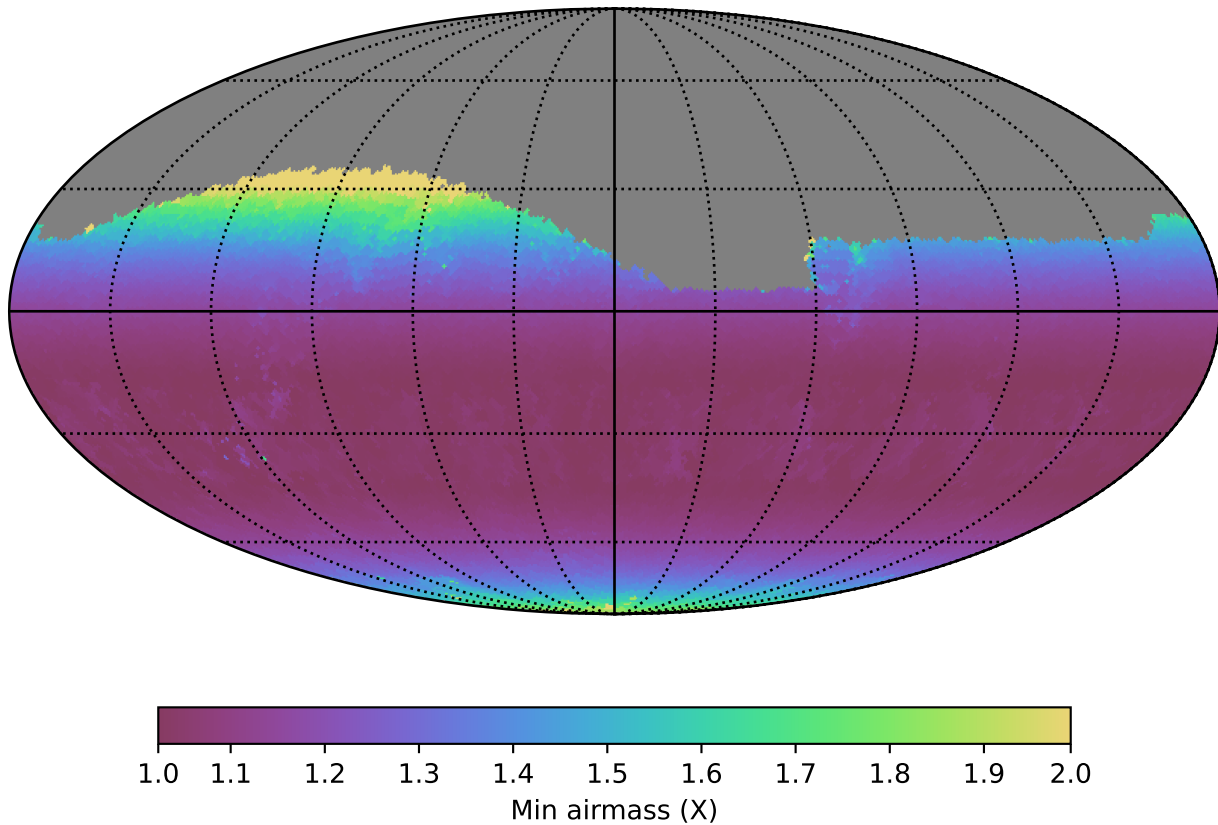
telescope_jerk_v3.5_10yrs Yr 1 r band: Min airmass
