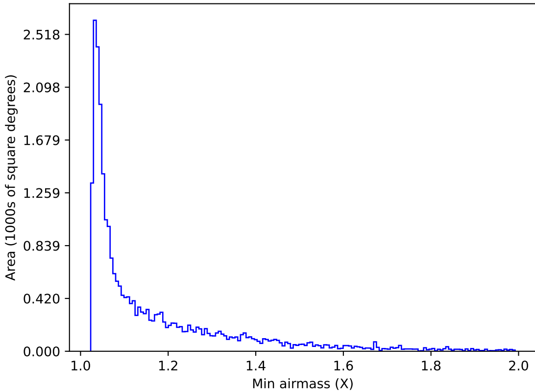
telescope_jerk_v3.5_10yrs Yr 1 r band: Min airmass
