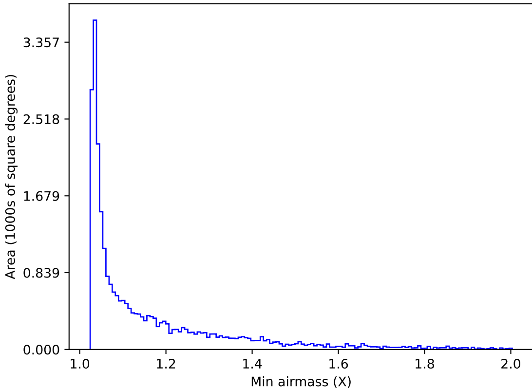
telescope_jerk_v3.5_10yrs Yr 1 i band: Min airmass
