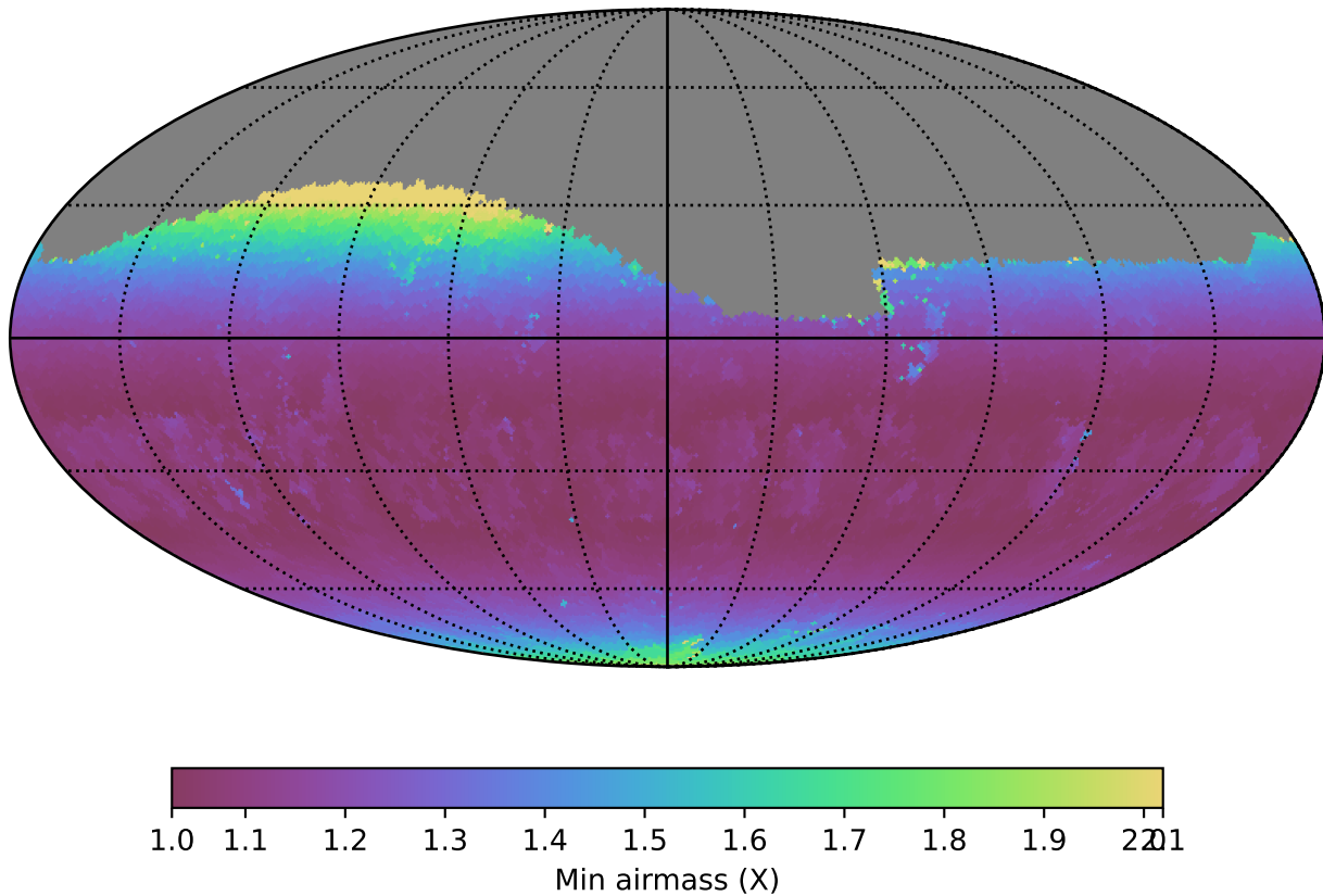
telescope_jerk_v3.5_10yrs Yr 1 g band: Min airmass
