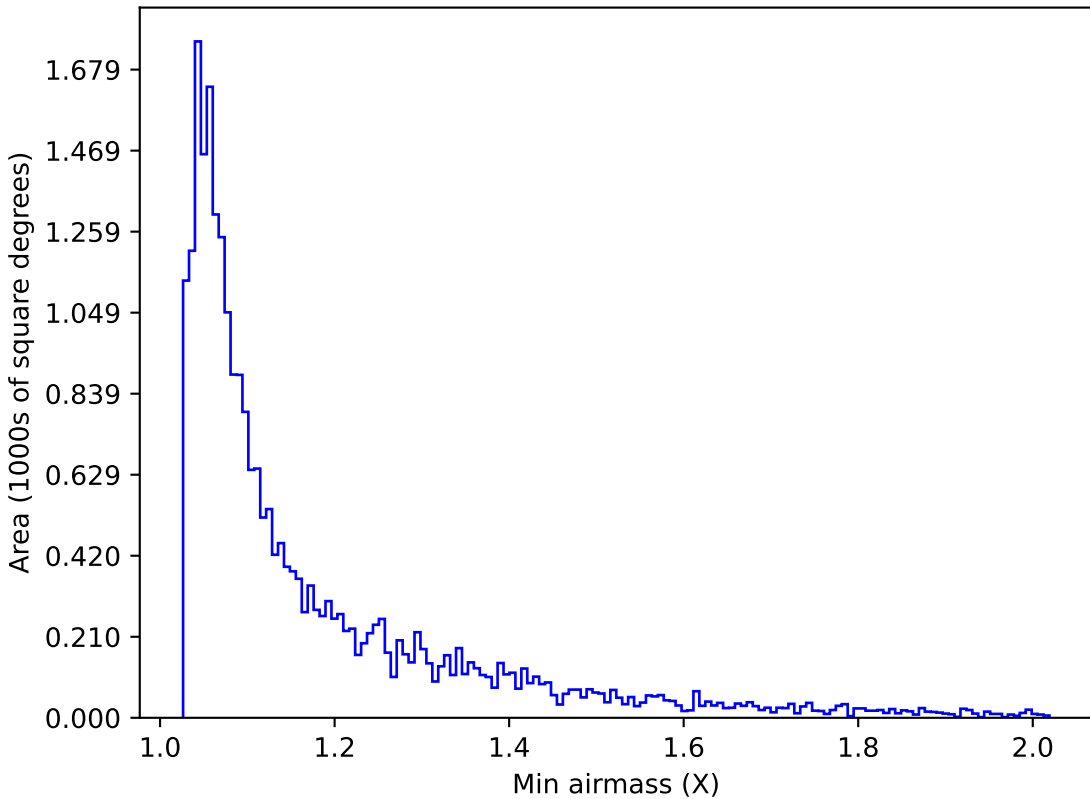
telescope_jerk_v3.5_10yrs Yr 1 g band: Min airmass
