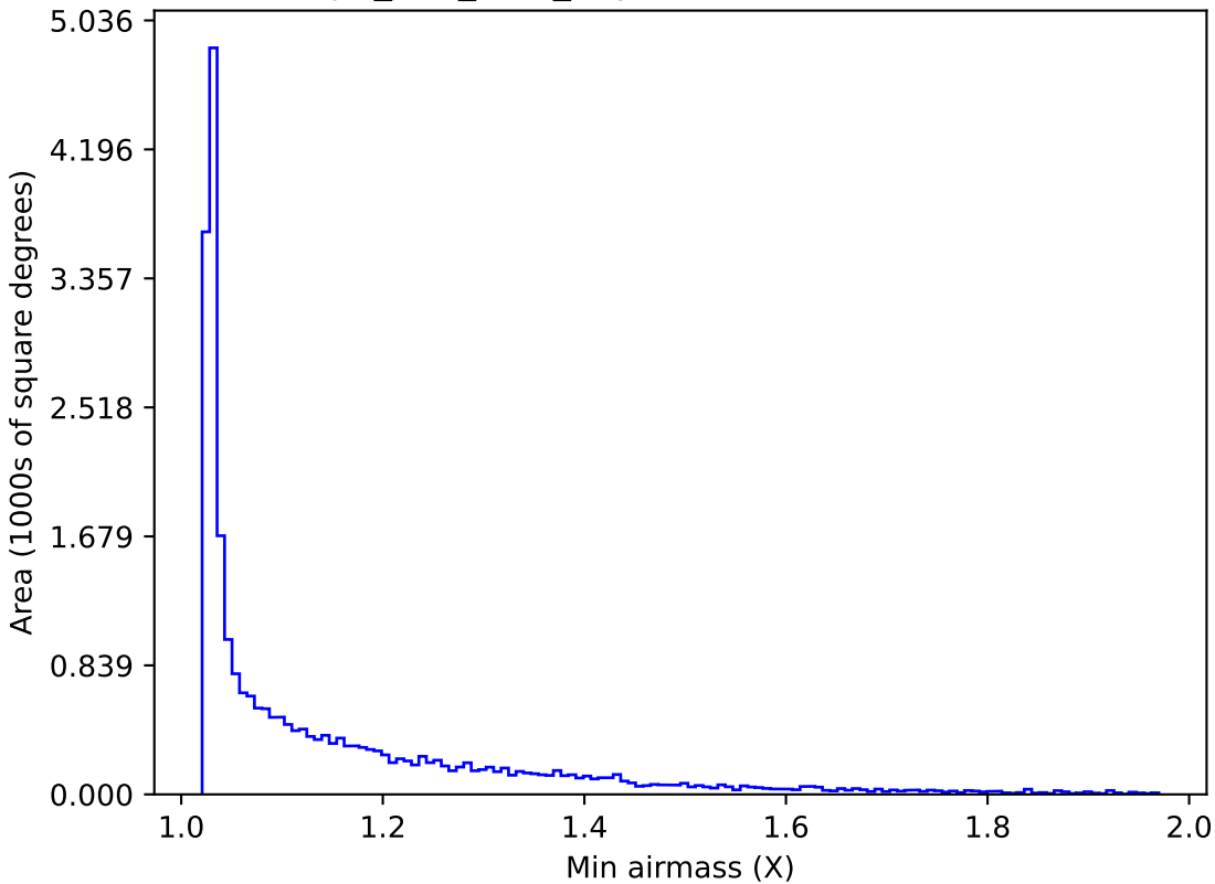
telescope_jerk_v3.5_10yrs Yr 1 all bands: Min airmass
