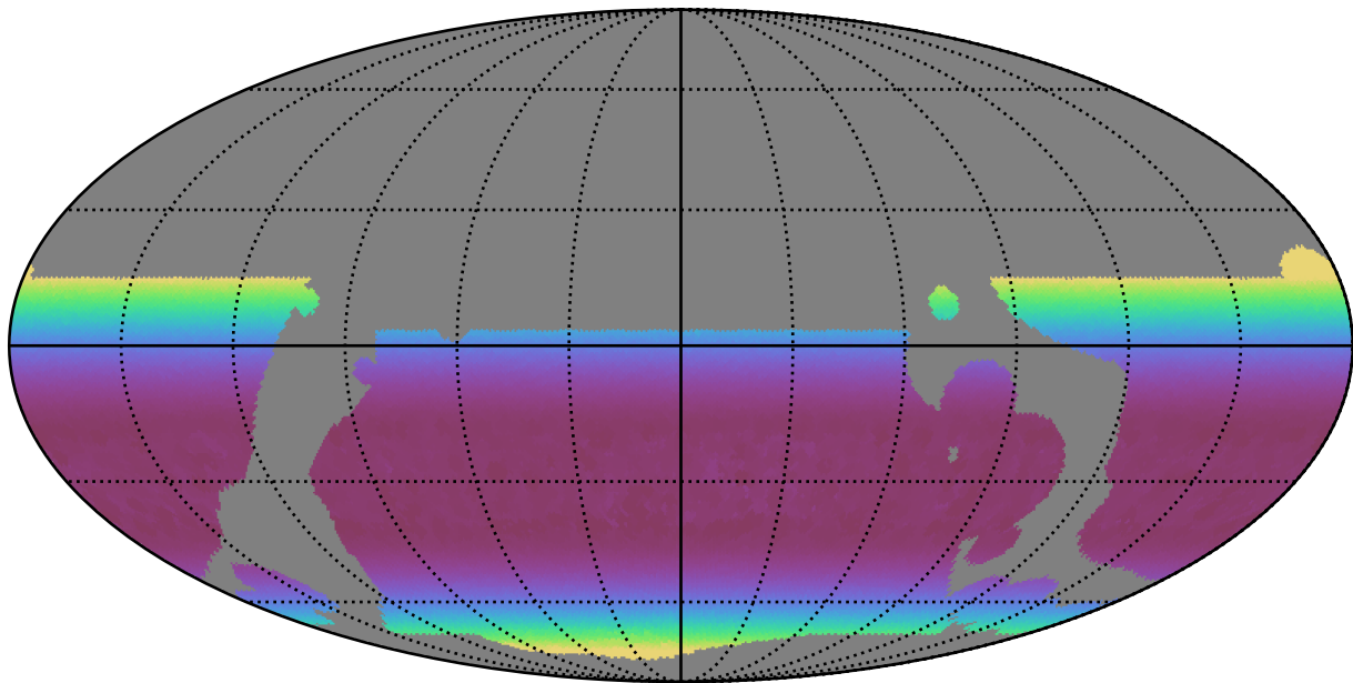
telescope_jerk_v3.5_10yrs WFD z band: Min airmass
