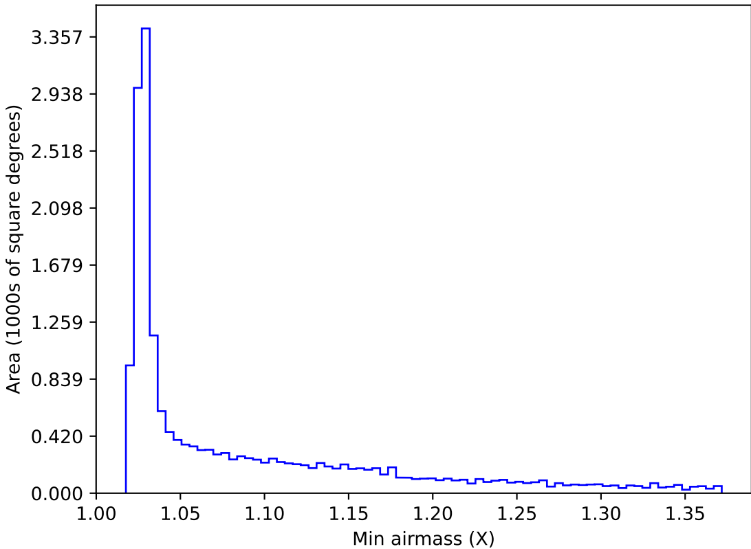
telescope_jerk_v3.5_10yrs WFD z band: Min airmass
