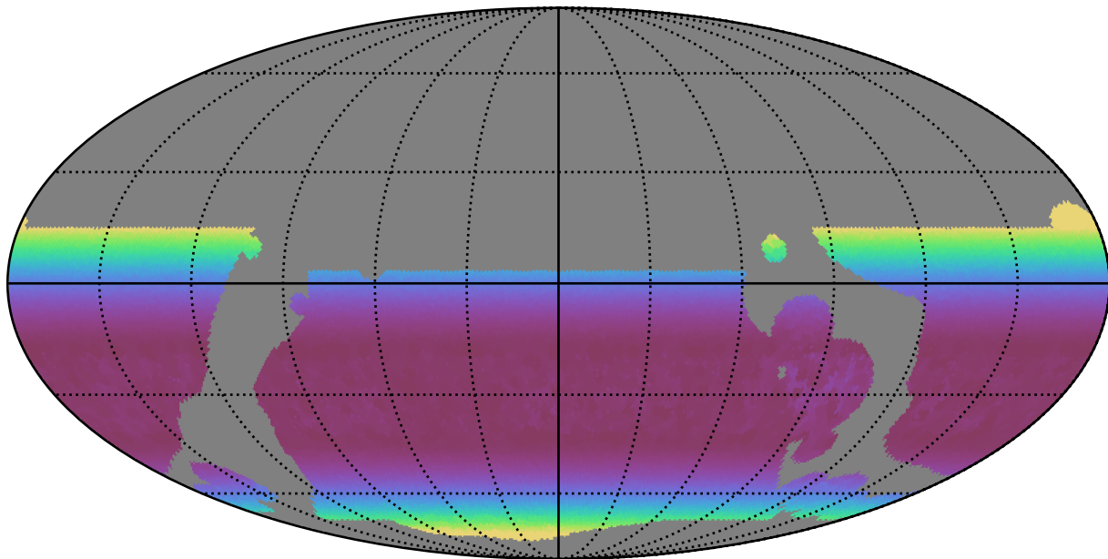
telescope_jerk_v3.5_10yrs WFD y band: Min airmass
