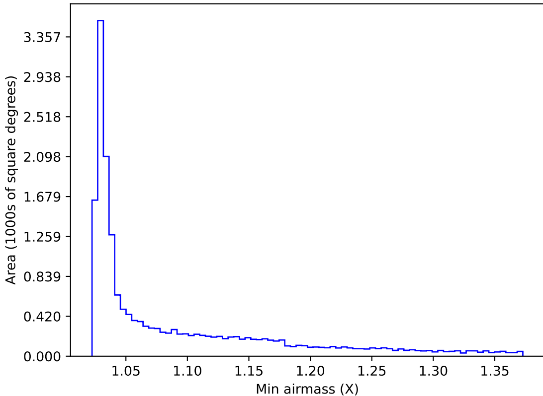
telescope_jerk_v3.5_10yrs WFD y band: Min airmass
