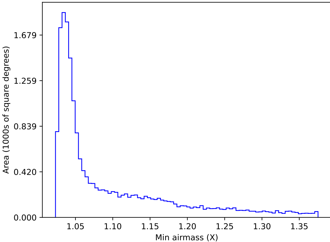
telescope_jerk_v3.5_10yrs WFD u band: Min airmass
