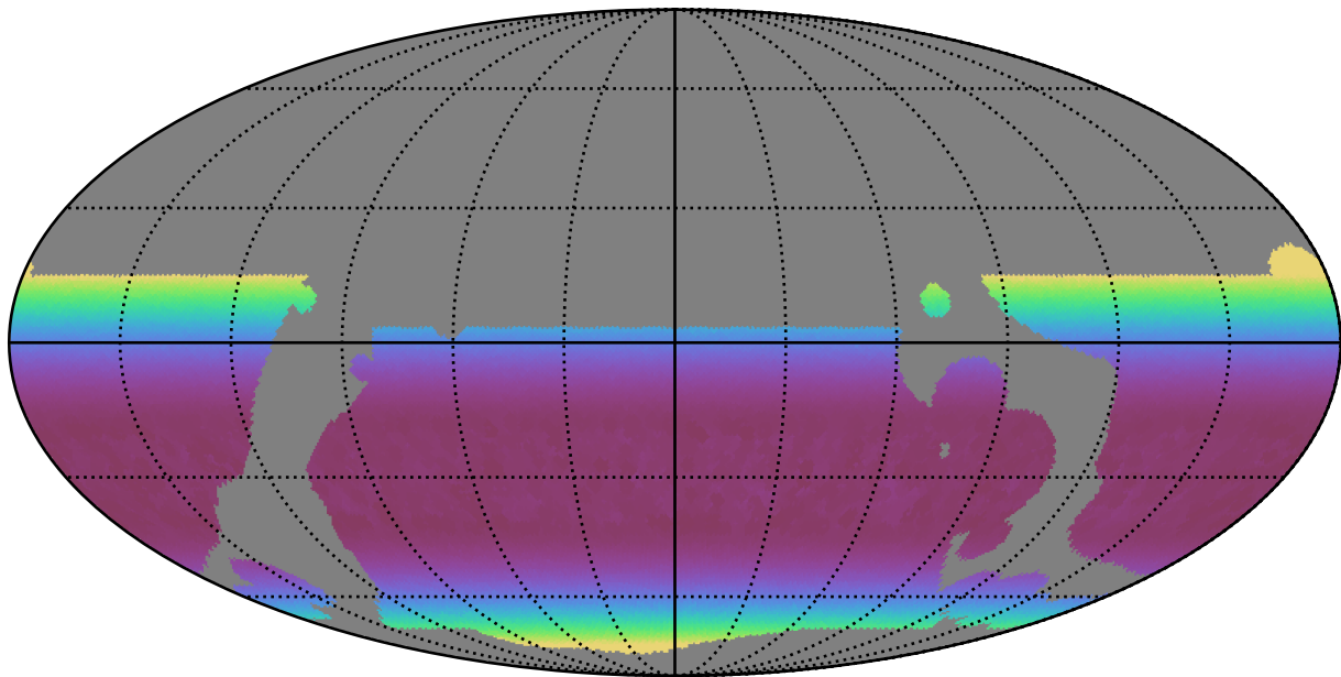
telescope_jerk_v3.5_10yrs WFD r band: Min airmass
