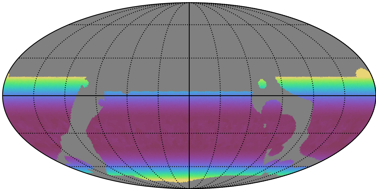
telescope_jerk_v3.5_10yrs WFD i band: Min airmass
