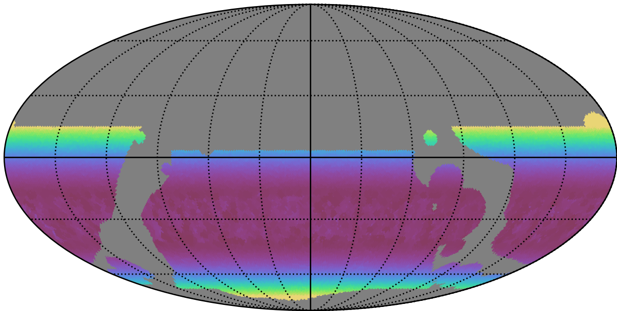
telescope_jerk_v3.5_10yrs WFD g band: Min airmass
