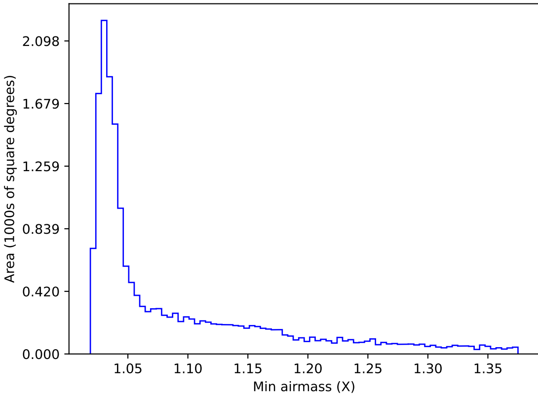
telescope_jerk_v3.5_10yrs WFD g band: Min airmass
