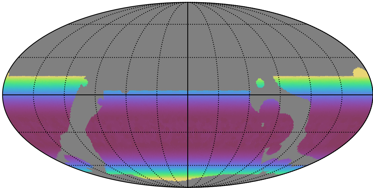
telescope_jerk_v3.5_10yrs WFD all bands: Min airmass
