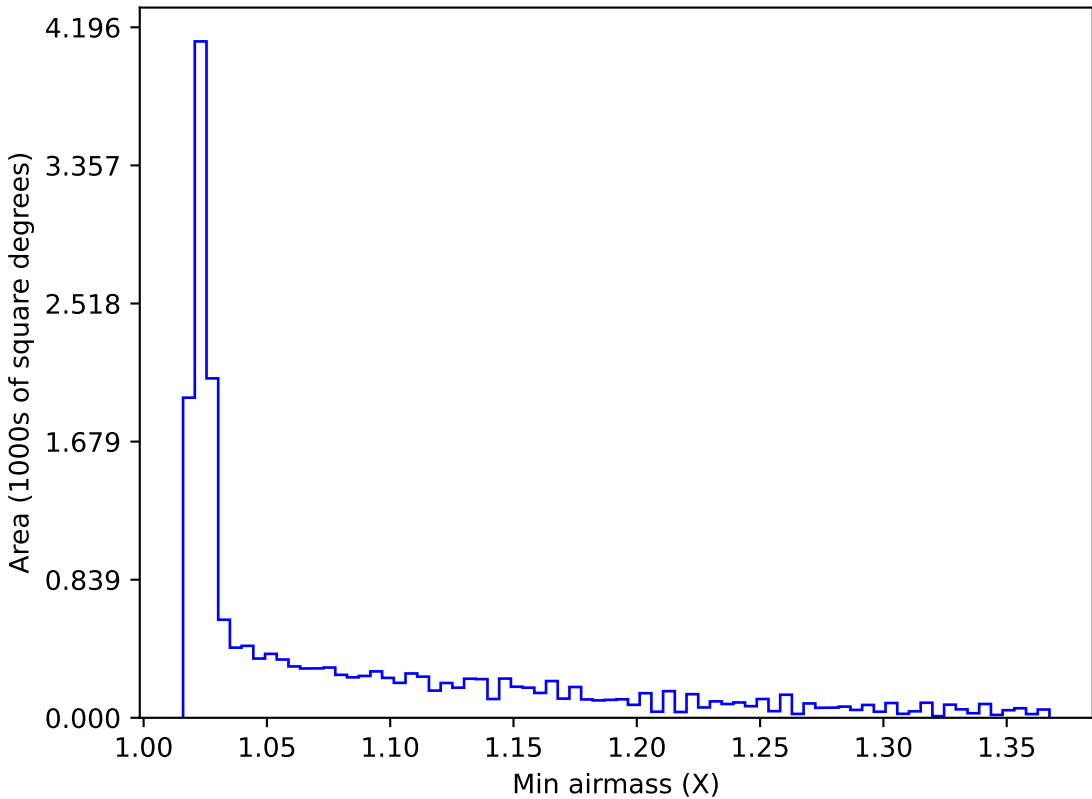
telescope_jerk_v3.5_10yrs WFD all bands: Min airmass
