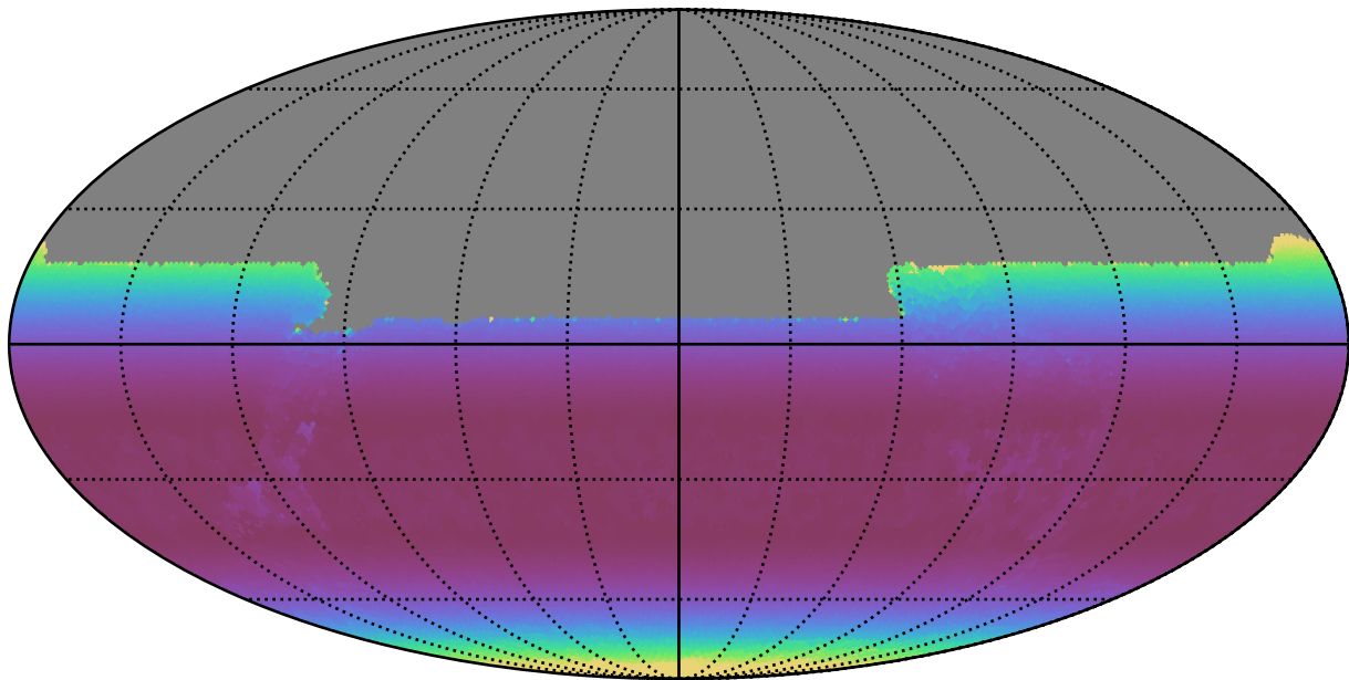
telescope_jerk_v3.5_10yrs All sky y band: Min airmass
