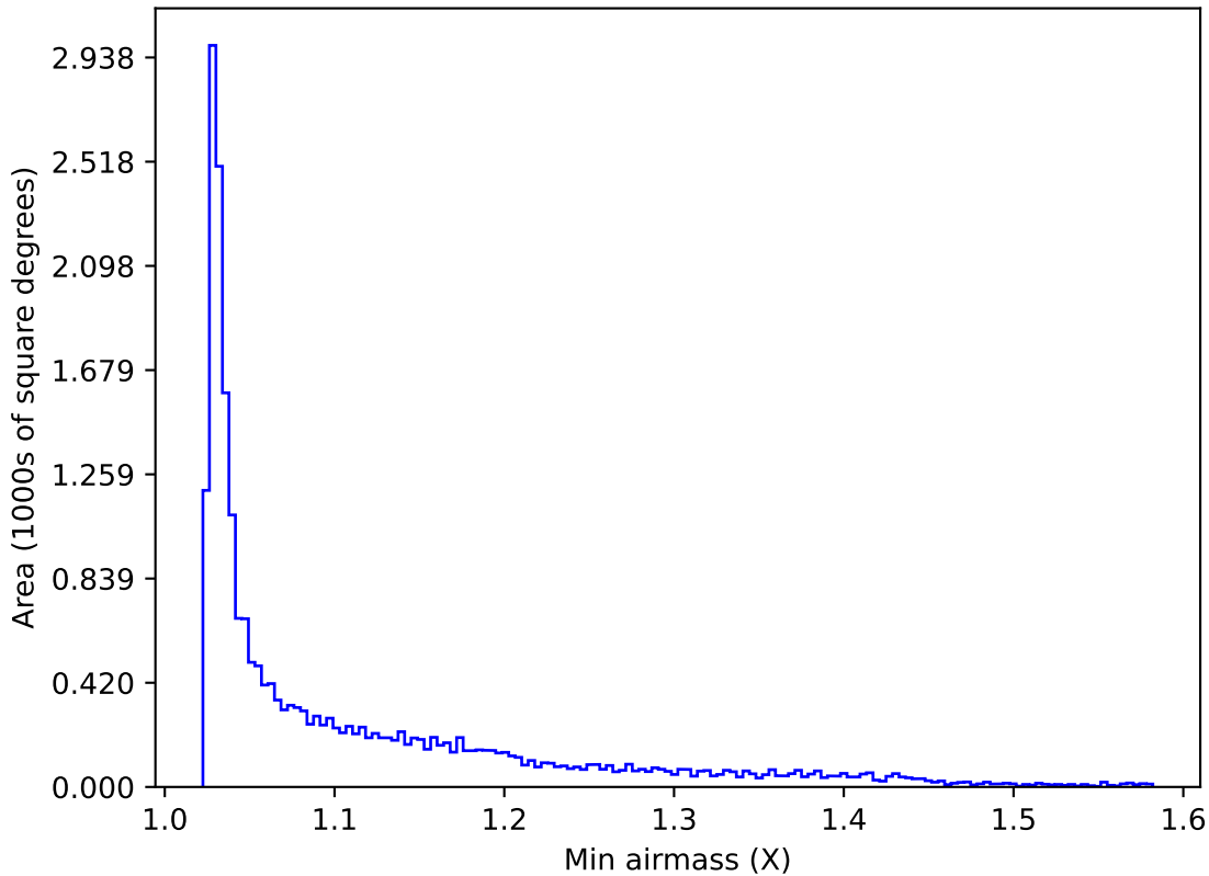
telescope_jerk_v3.5_10yrs All sky y band: Min airmass
