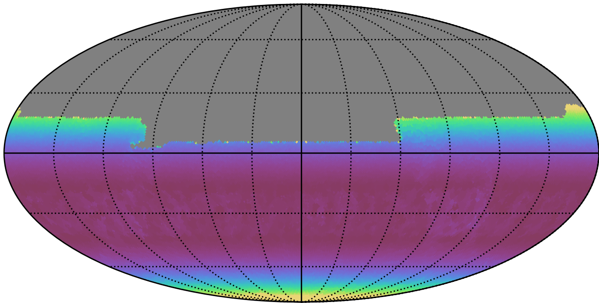
telescope_jerk_v3.5_10yrs All sky u band: Min airmass
