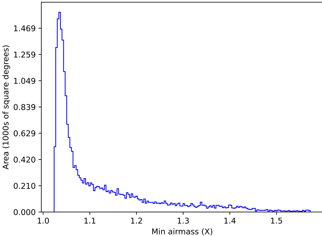
telescope_jerk_v3.5_10yrs All sky u band: Min airmass
