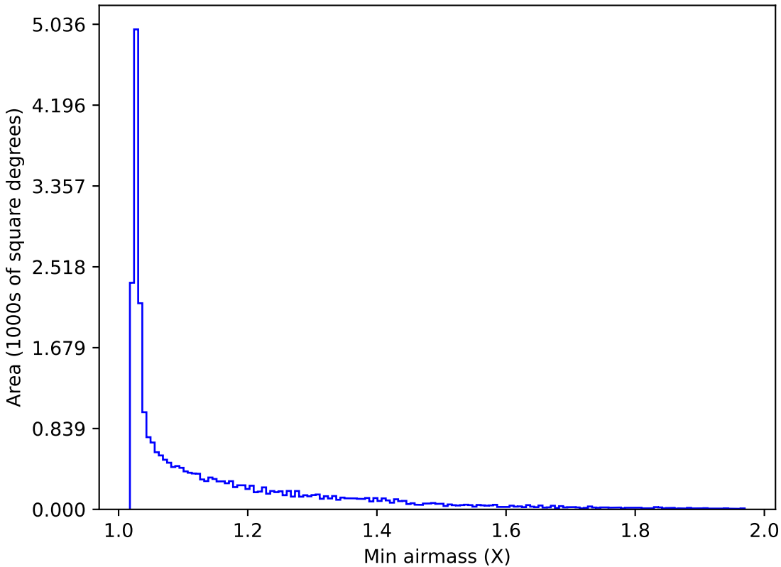
telescope_jerk_v3.5_10yrs All sky r band: Min airmass
