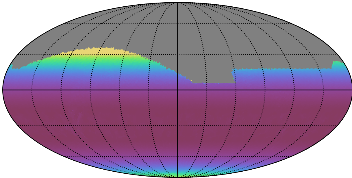
telescope_jerk_v3.5_10yrs All sky i band: Min airmass
