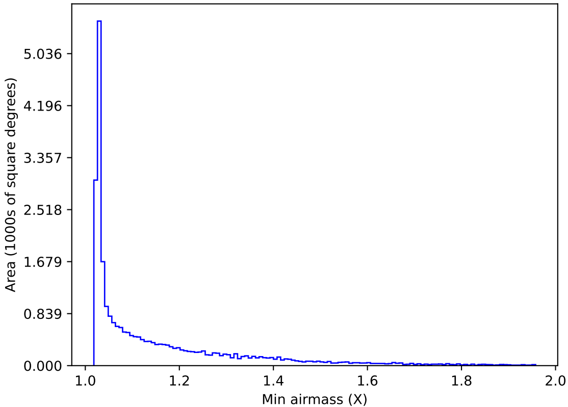
telescope_jerk_v3.5_10yrs All sky i band: Min airmass
