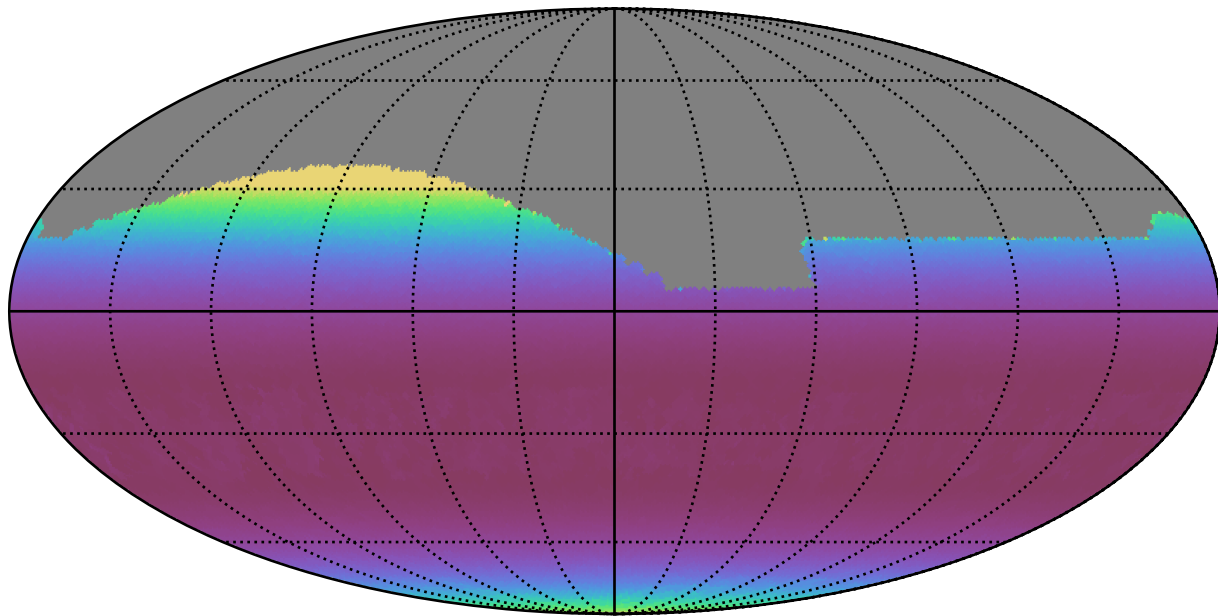
telescope_jerk_v3.5_10yrs All sky g band: Min airmass
