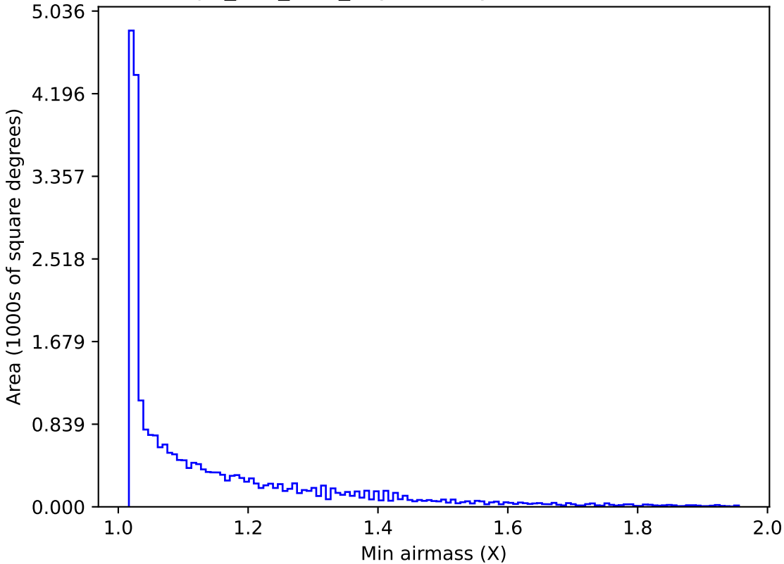
telescope_jerk_v3.5_10yrs All sky all bands: Min airmass
