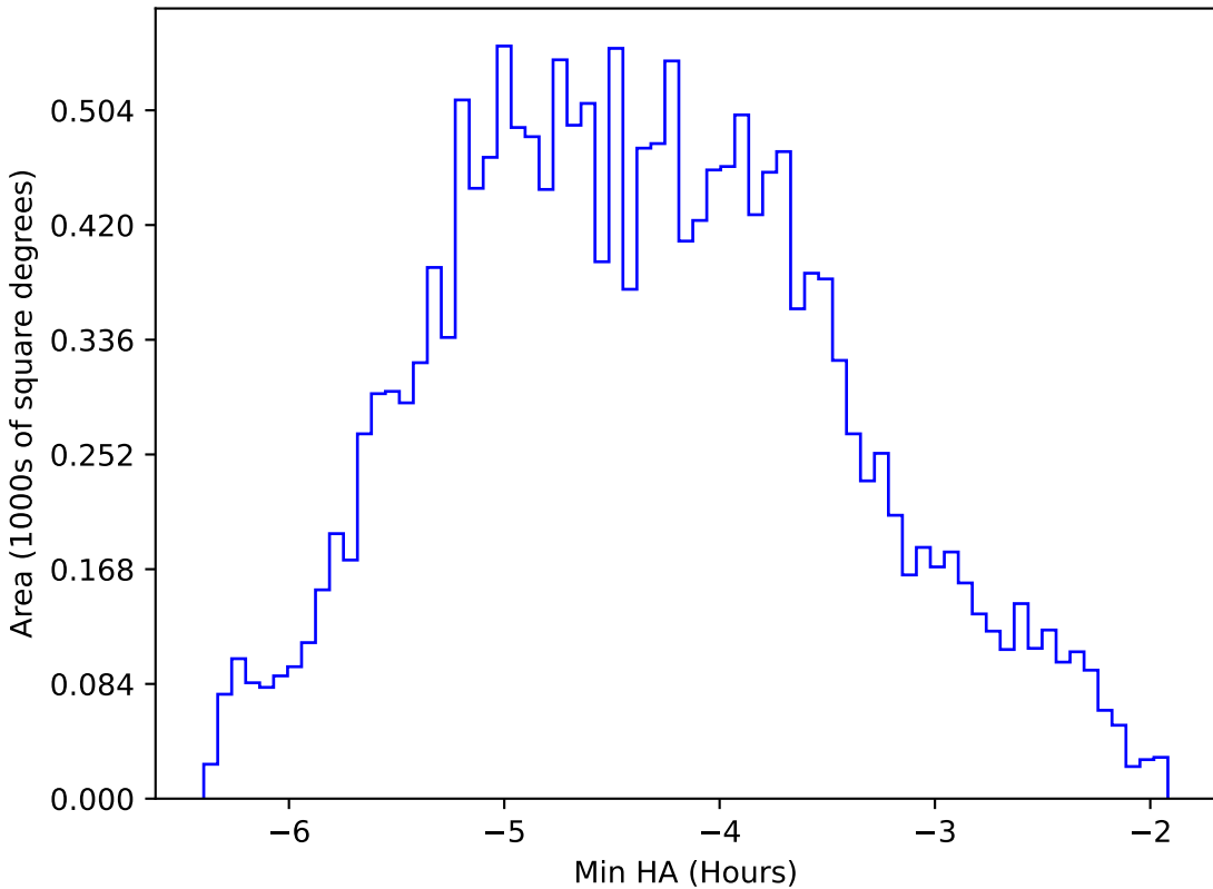
telescope_jerk_v3.5_10yrs WFD z band: Min HA
