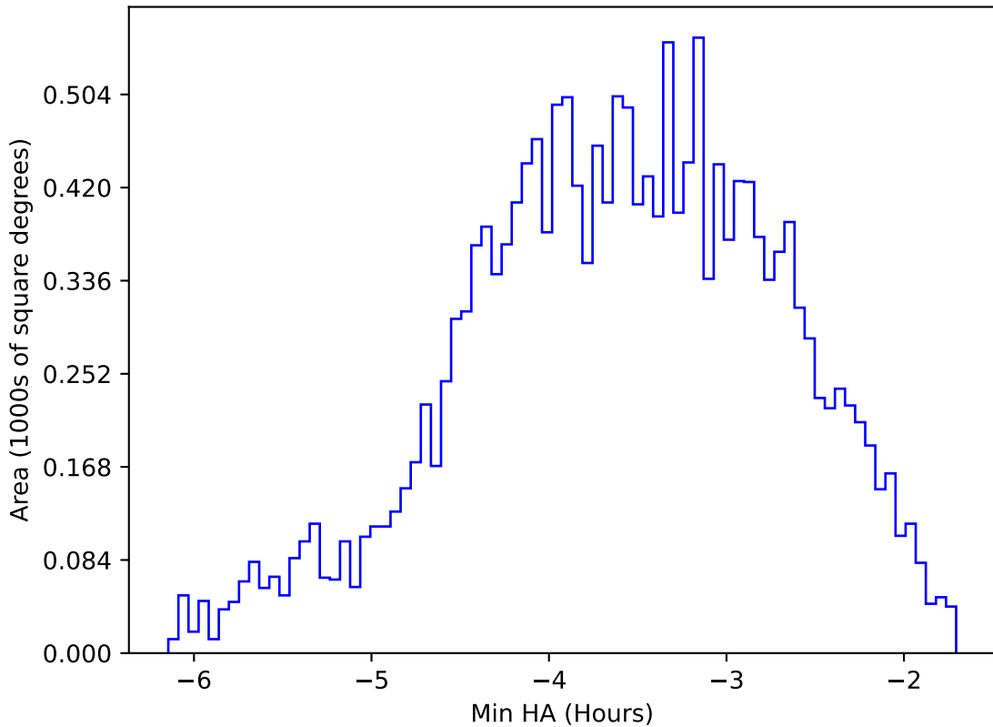
telescope_jerk_v3.5_10yrs WFD y band: Min HA
