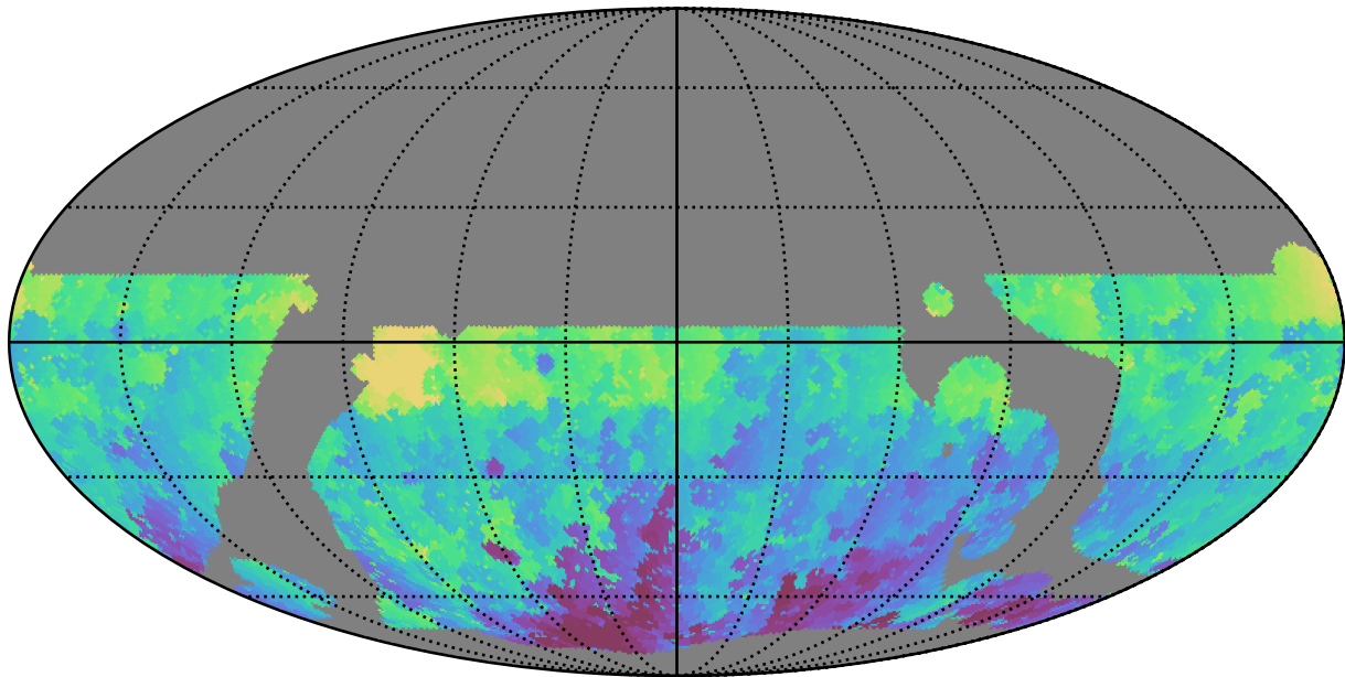
telescope_jerk_v3.5_10yrs WFD u band: Min HA
