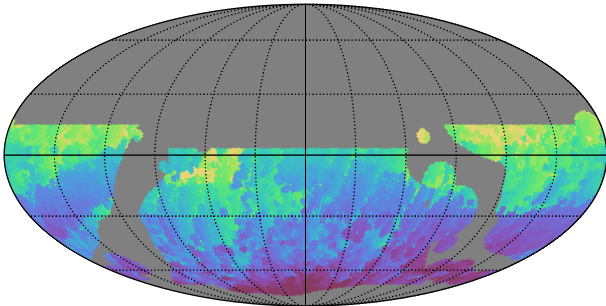
telescope_jerk_v3.5_10yrs WFD r band: Min HA
